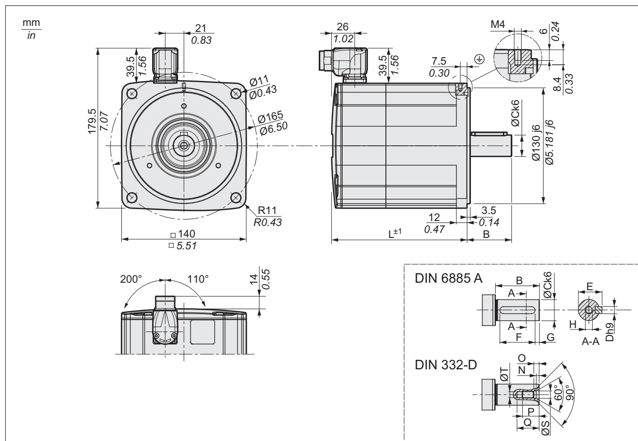
Figure 5: Dimensions BMP140
