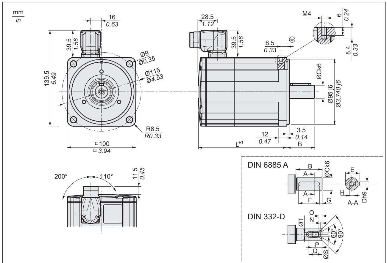
Figure 4: Dimensions BMP100
